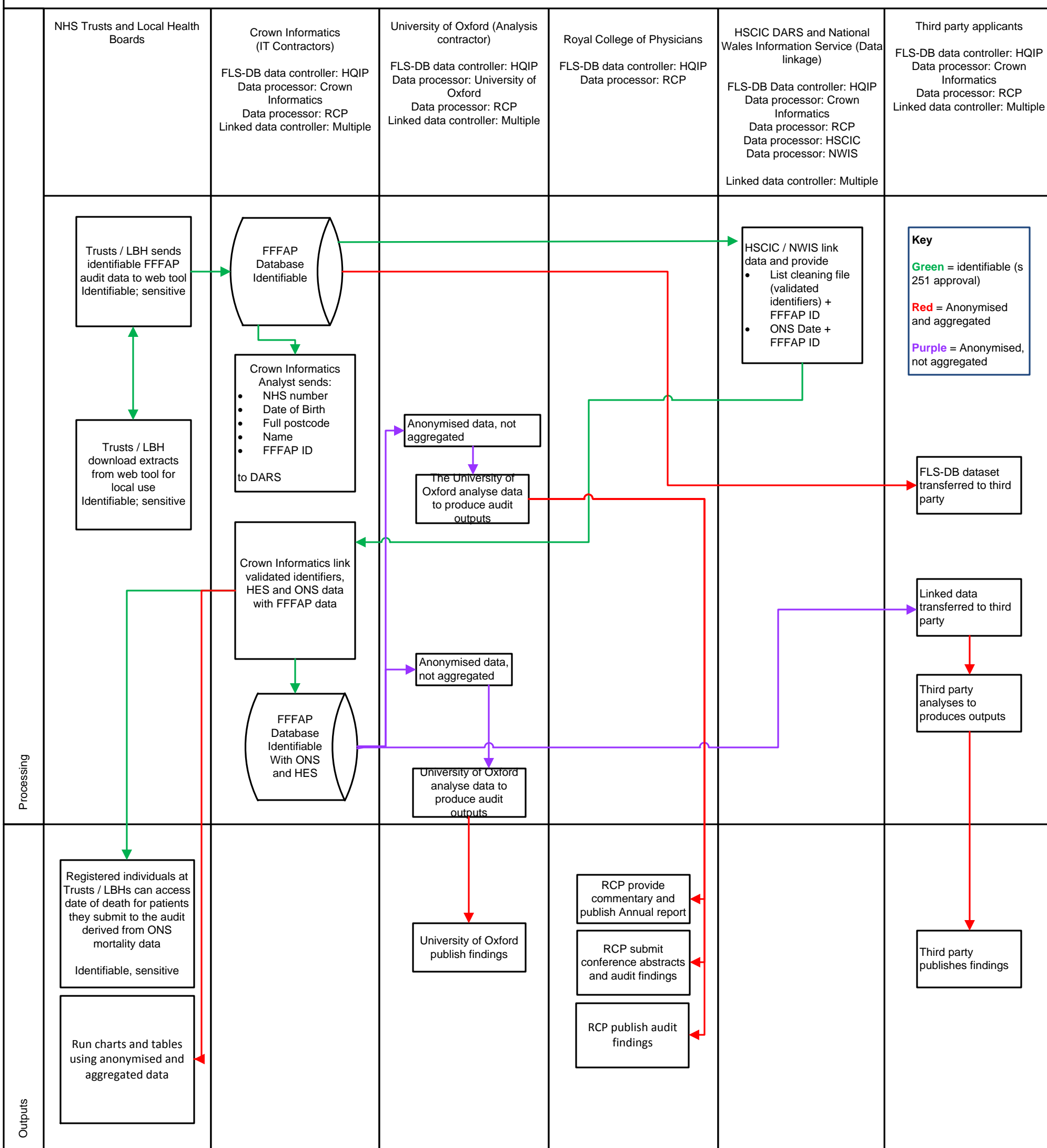
Falls and Fragility Audit Programme: Fracture Liaison Service Database (FLS-DB) data flow diagram
