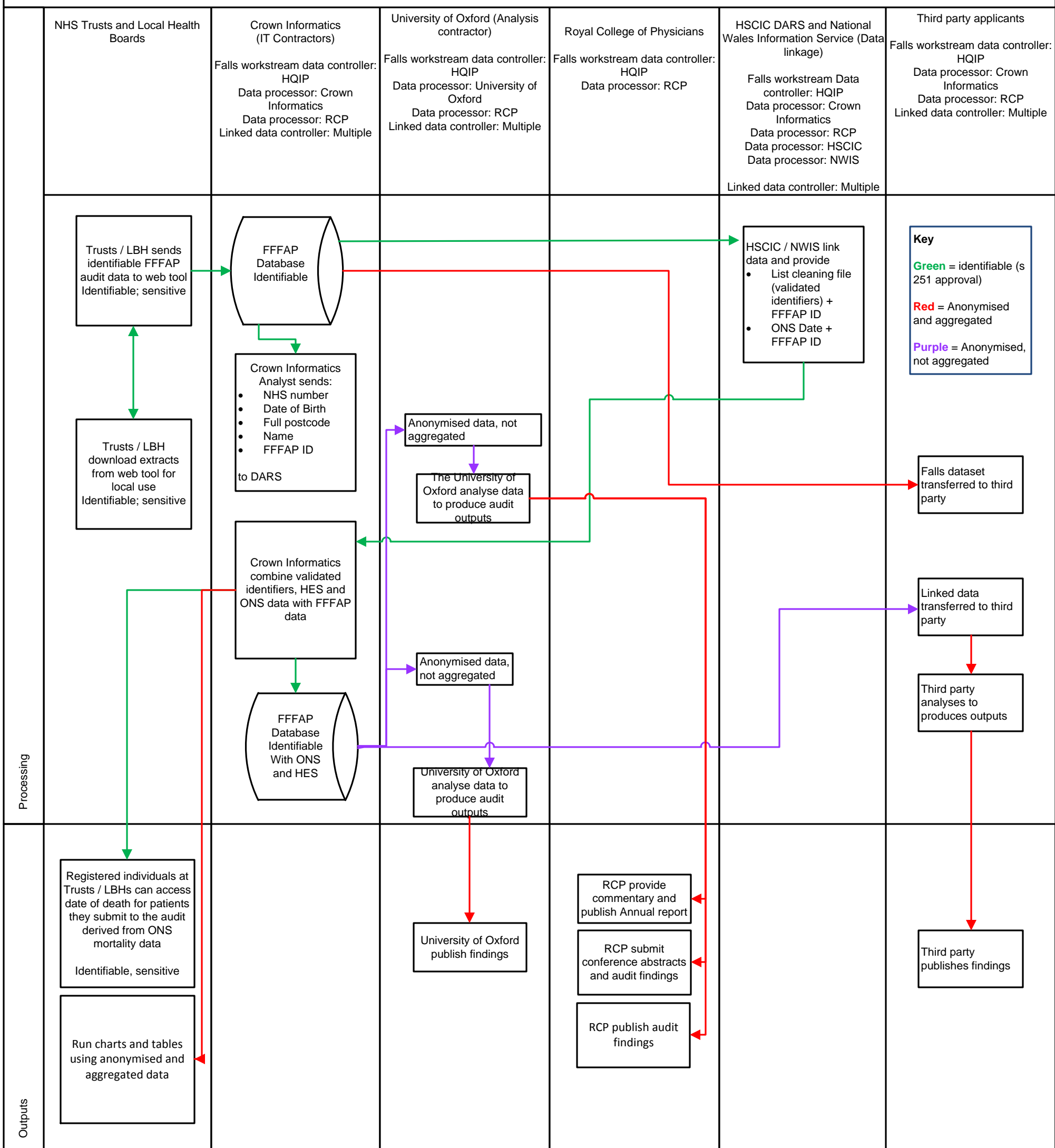
Falls and Fragility Audit Programme: Falls workstream data flow diagram
